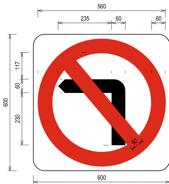
NO LEFT TURN
