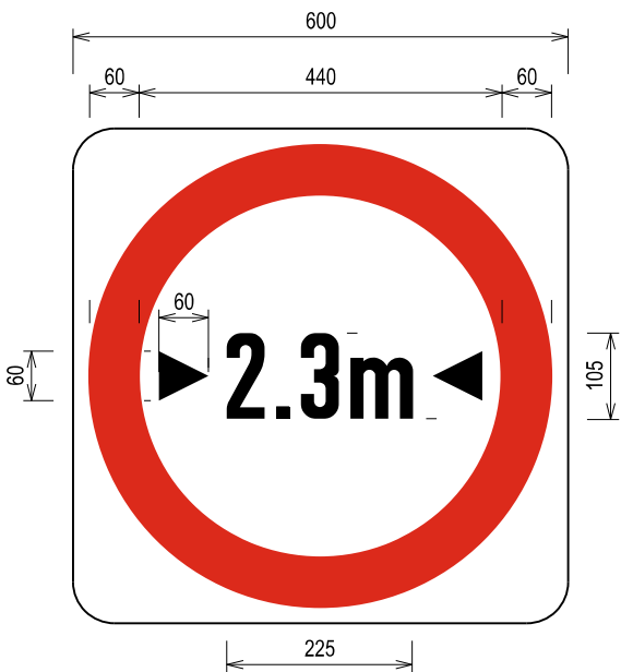
WIDTH LIMIT
