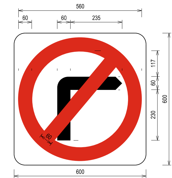
NO RIGHT TURN
