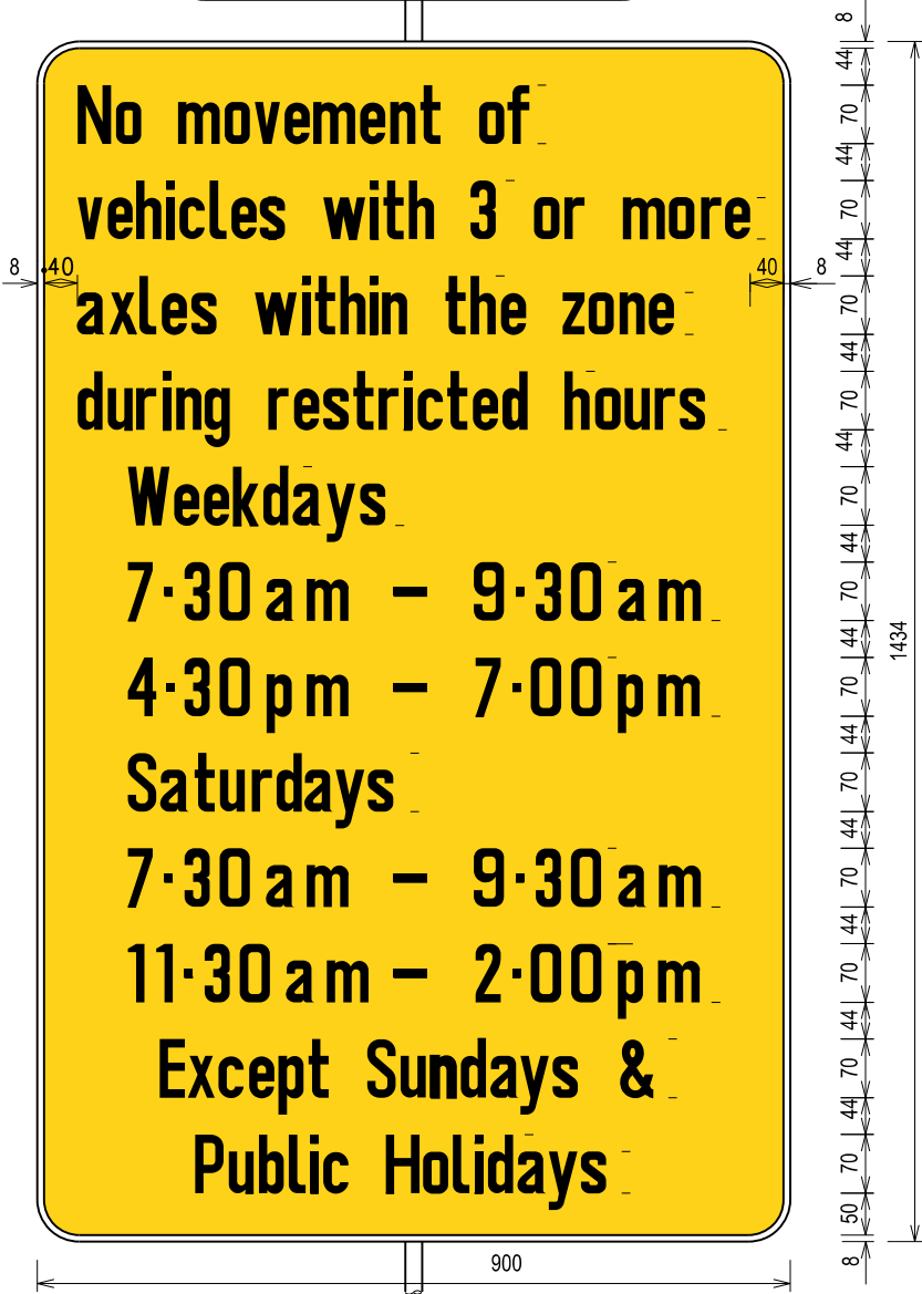
RESTRICTION OF MOVEMENT OF VEHICLES WITH 3 OR MORE AXLES.
